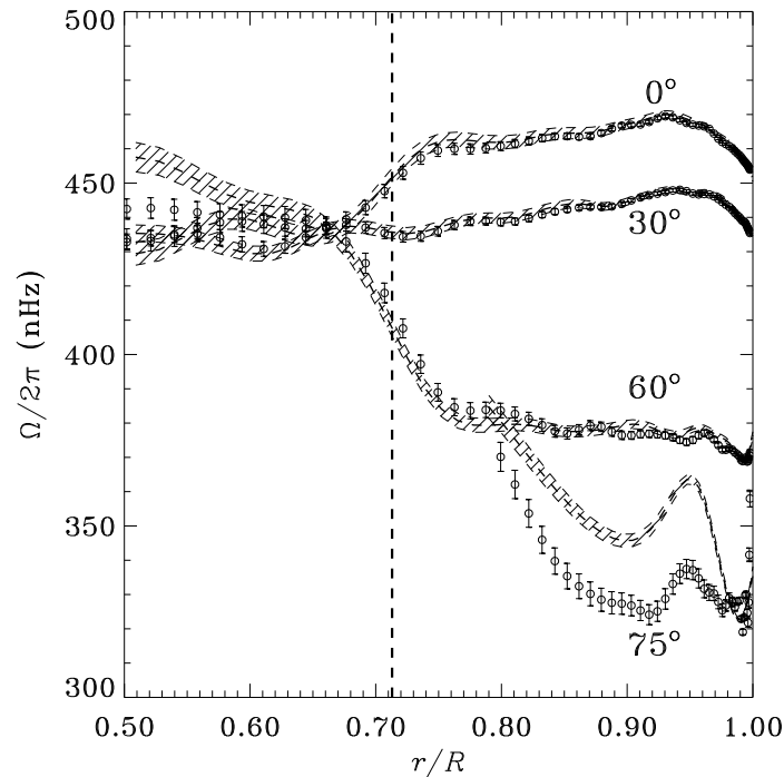
Figure 9.8: Inferred rotation rate \Omega/2\pi as a function of radius at the latitudes indicated, obtained from inversion of 144 days of MDI data. The circles with 1- \sigma error bars show results of a SOLA inversion, while the dashed lines with 1- \sigma error band were obtained with regularized least-squares inversion. The heavy vertical dashed line marks the base of the convection zone. (Adapted from Schou et al. , 1998.)
