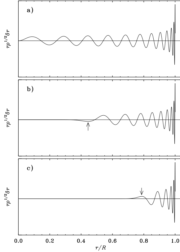
Figure 5.8: Scaled radial displacement eigenfunctions for selected p modes in a normal solar model, with a) l = 0 , n = 23 , \nu = 3310 \mu\text{Hz} ; b) l = 20 , n = 17 , \nu = 3375 \mu\text{Hz} ; c) l = 60 , n = 10 , \nu = 3234 \mu\text{Hz} . The arrows mark the asymptotic location of the turning points r_t [cf. equation (5.28)].
