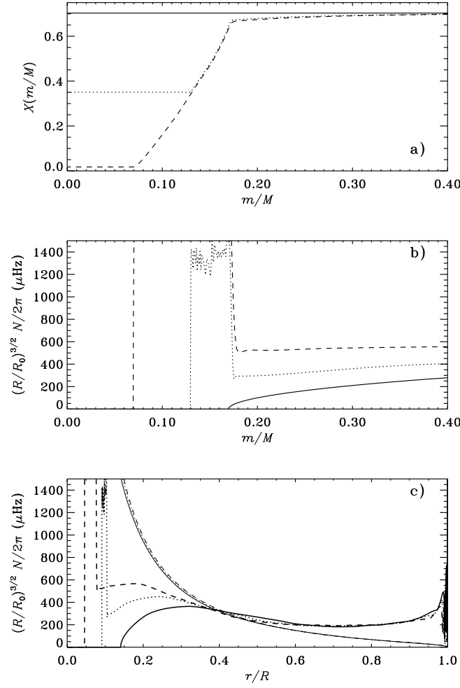
Figure 5.3: (a) Hydrogen content X against mass fraction m/M for three models in a 2.2M_\odot evolution sequence. The solid line is for age 0, the dotted line for age 0.47 Gyr and the dashed line for age 0.71 Gyr. Only the inner 40 per cent of the models is shown. (b) Scaled buoyancy frequency, expressed in terms of cyclic frequency, against m/M for the same three models. In the scaling factor, R and R_0 are the radii of the actual and the zero-age main sequence model, respectively. For the model of age 0.71 Gyr, the maximum value of (R/R_0)^{3/2}N/2\pi is 2400\mu\text{Hz} . (c) Scaled buoyancy frequency N (heavy lines) and characteristic acoustic frequency S_l for l=2 (thin lines), for the same three models, plotted against fractional radius r/R .
