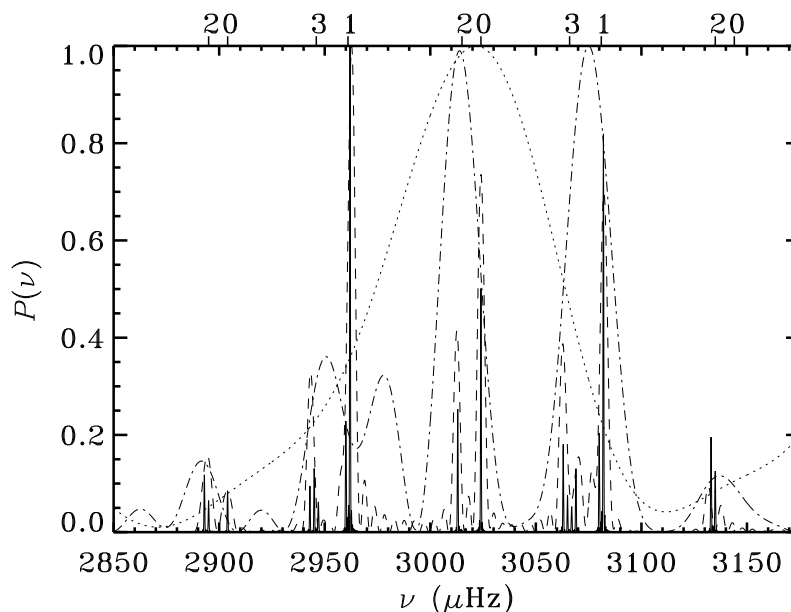
Figure 2.7: Power spectra of simulated time series of duration 600 h (—), 60 h (-----), 10 h (-·-·-·-) and 3 h (·····). The power is on an arbitrary scale and has been normalized to a maximum value of 1. The location of the central frequency for each group of rotationally split modes, as well as the value of the degree, are indicated on the top of the diagram. (From Christensen-Dalsgaard 1984b.)
