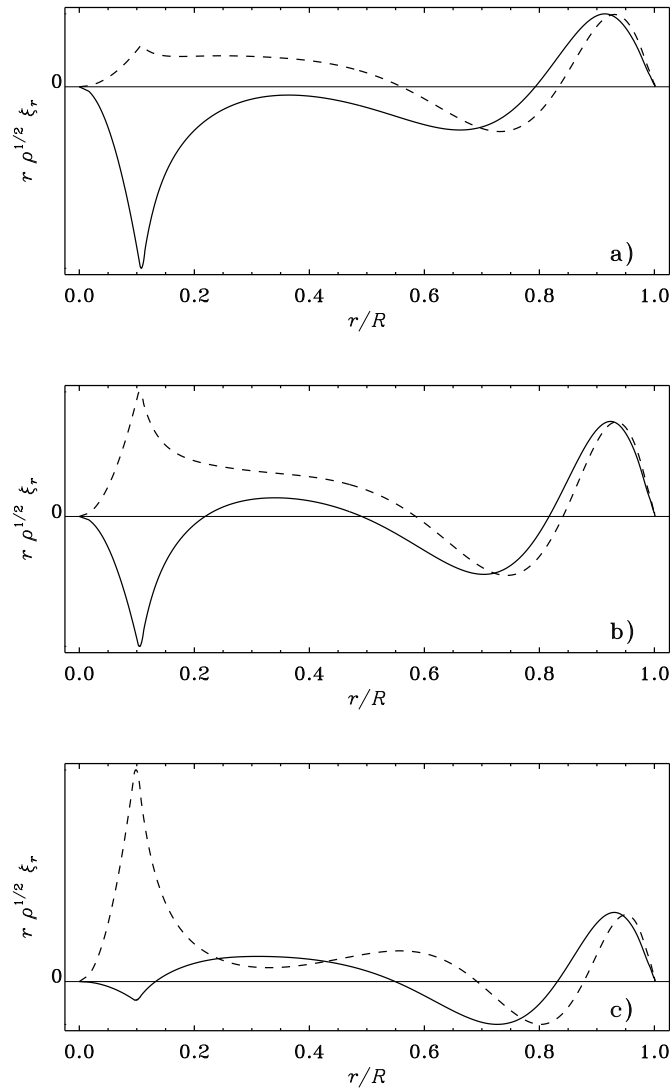
Figure 5.15: Scaled eigenfunctions for the p_1(l=2) mode (continuous line) and the p_2(l=2) mode (dashed line) in the vicinity of the avoided crossing near age 0.4 Gyr, (R/R_0)^{3/2}\nu = 400 \mu\text{Hz} in Figure 5.14. (a) Age 0.36 Gyr. (b) Age 0.39 Gyr. (c) Age 0.44 Gyr.
